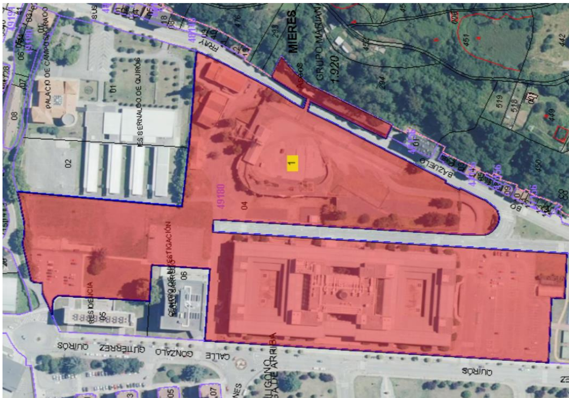
Figure 6-2. General view of and the new photovoltaic plant location projected.
