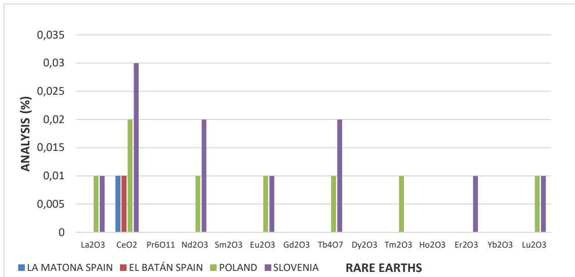
Figure 3-3. Graph of the percentage of initial analysis of oxides of rare earths
