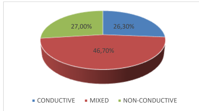
Figure 10-4. Different fractions resulting from the electrical separator of the La Matona sample
